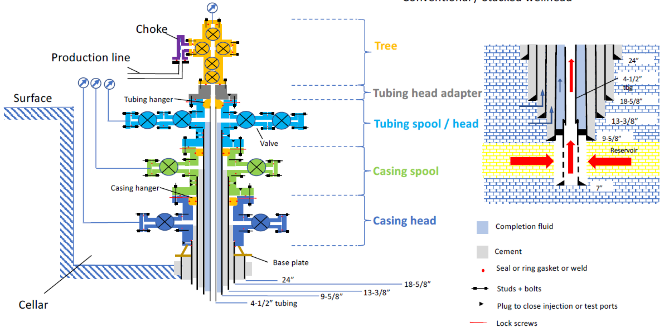
Conventional / Stacked wellhead
